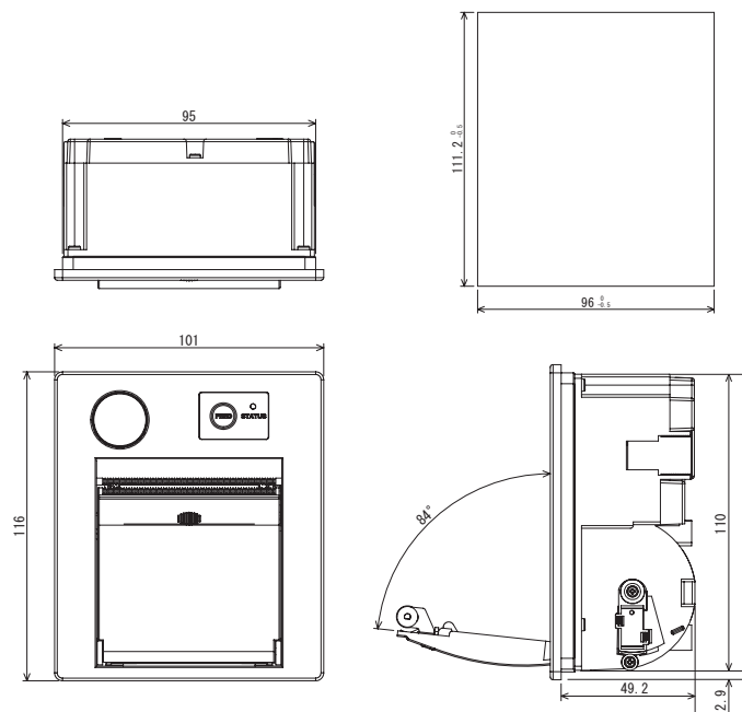
取付穴寸法/MOUNTING SIZE
