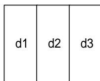
24-dot bitimage
